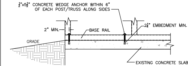
CONCRETE FOUNDATION/BASE RAIL ANCHOR DETAIL
