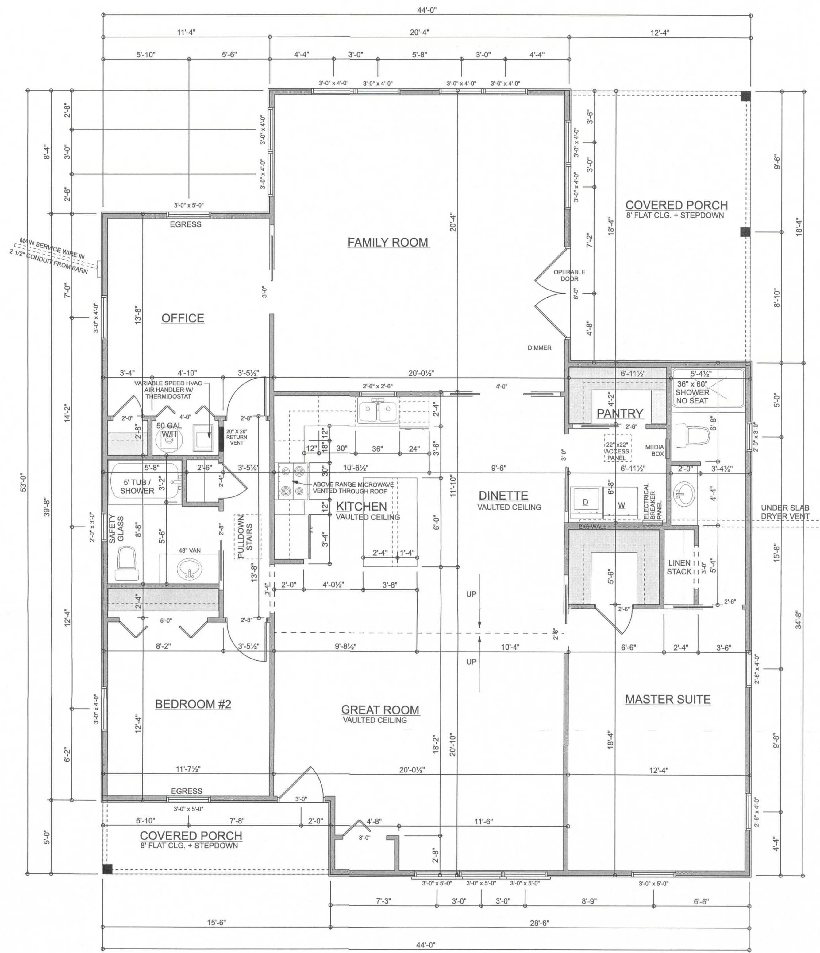
FLOOR PLAN SCALE: 1/4" = 1'-0" 8' FLAT CLG. UNLESS NOTED
