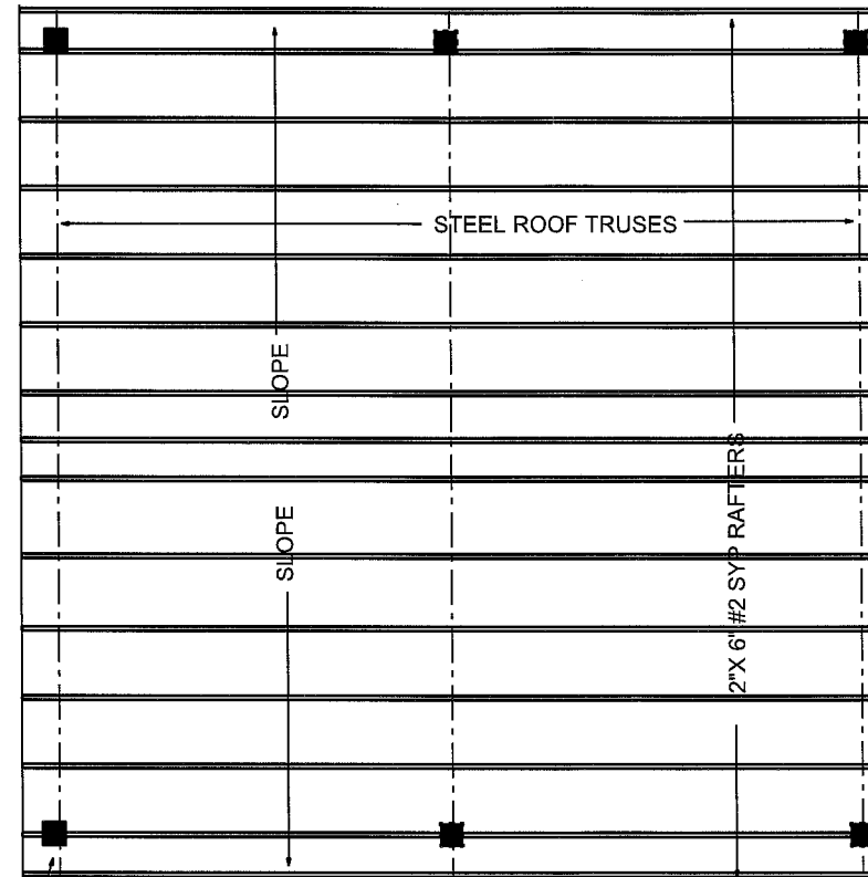
ROOF PLAN VIEW
