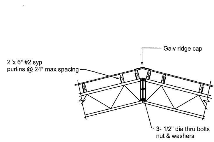
RIDGE CONNECTION DETAIL
