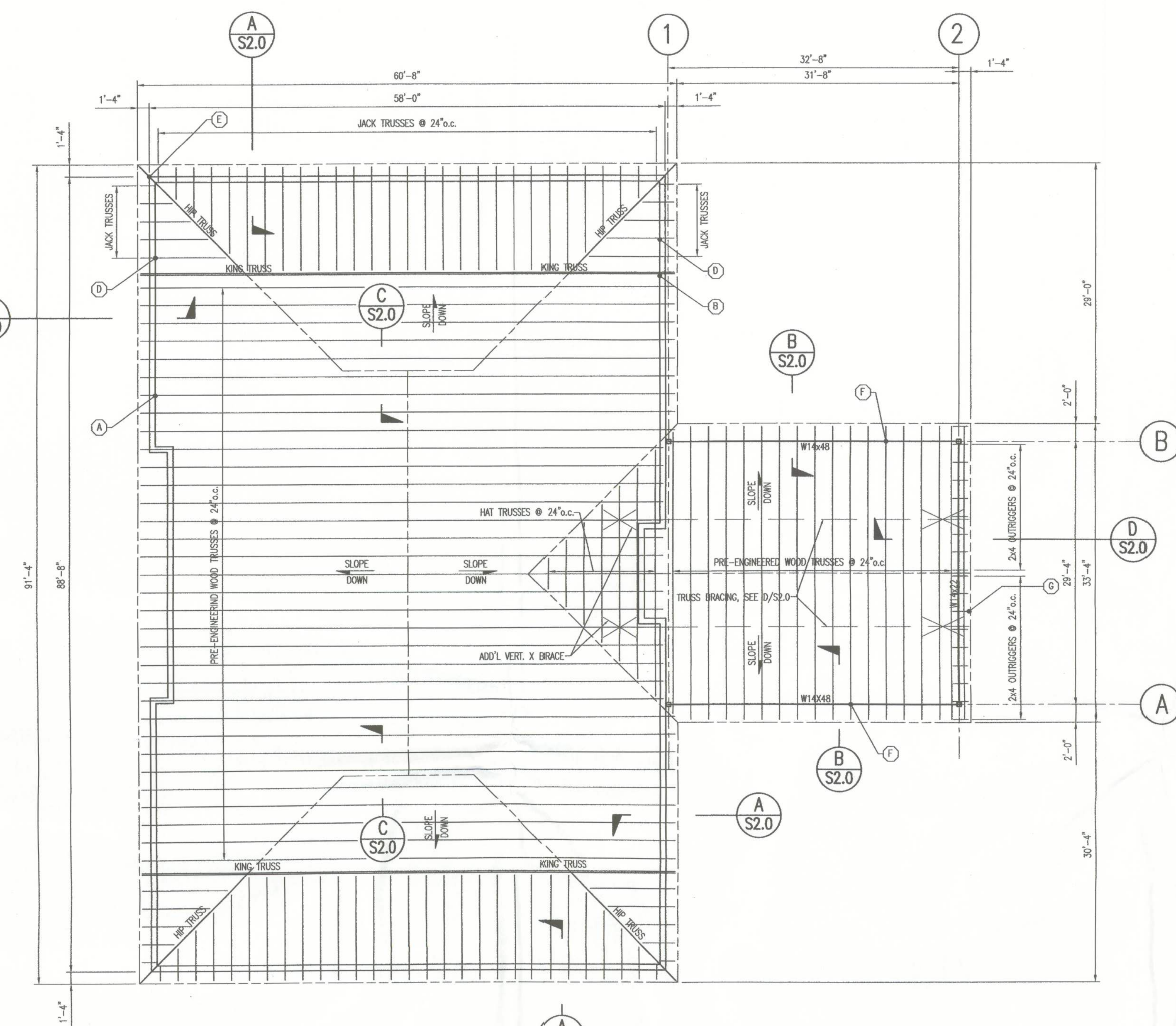
ROOF FRAMING PLAN SCALE: 3/8" = 1'-0"
