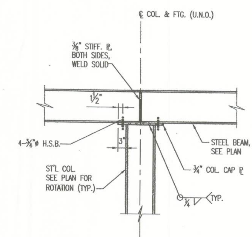
TYPICAL STEEL COLUMN CAP DETAIL NO SCALE
