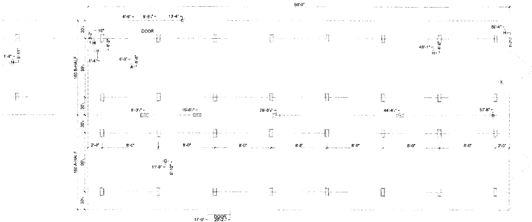
SUPPORT PIER/TYP. LOADING DESIGN VALUE—6420 lbs./PIER
