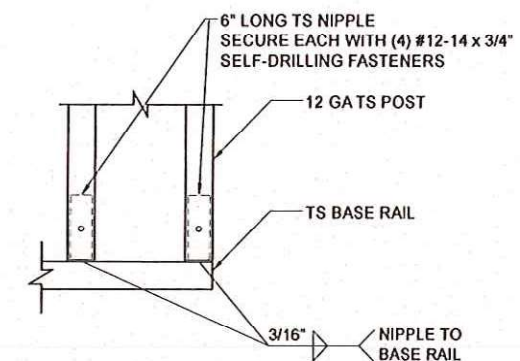
10 RAFTER POST/BASE BASE RAIL CONNECTION DETAIL Not To Scale
