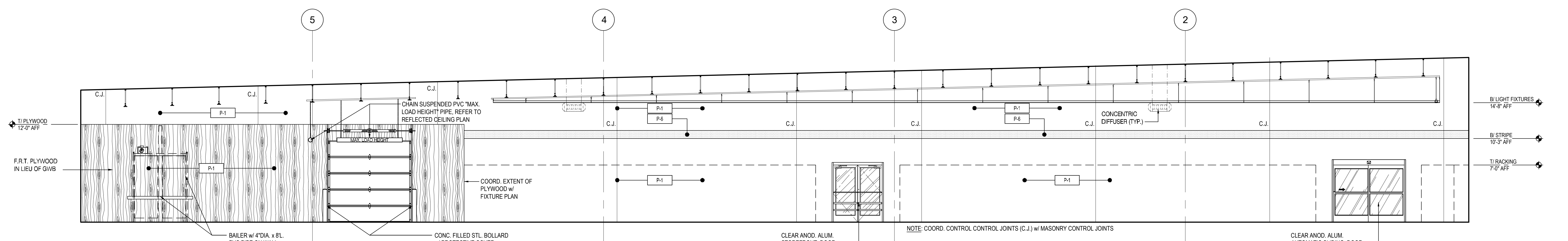
4 | INTERIOR ELEVATION 3/16"=1'-0"
