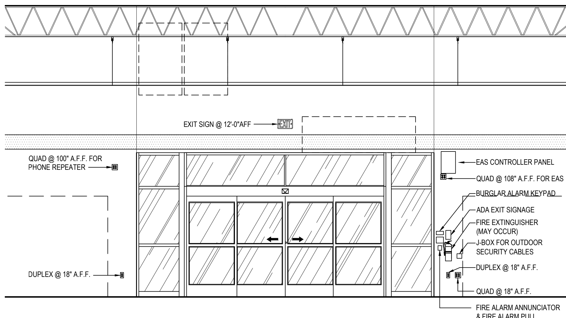
A | ENLARGED ELEVATION 1/4"=1'-0"
