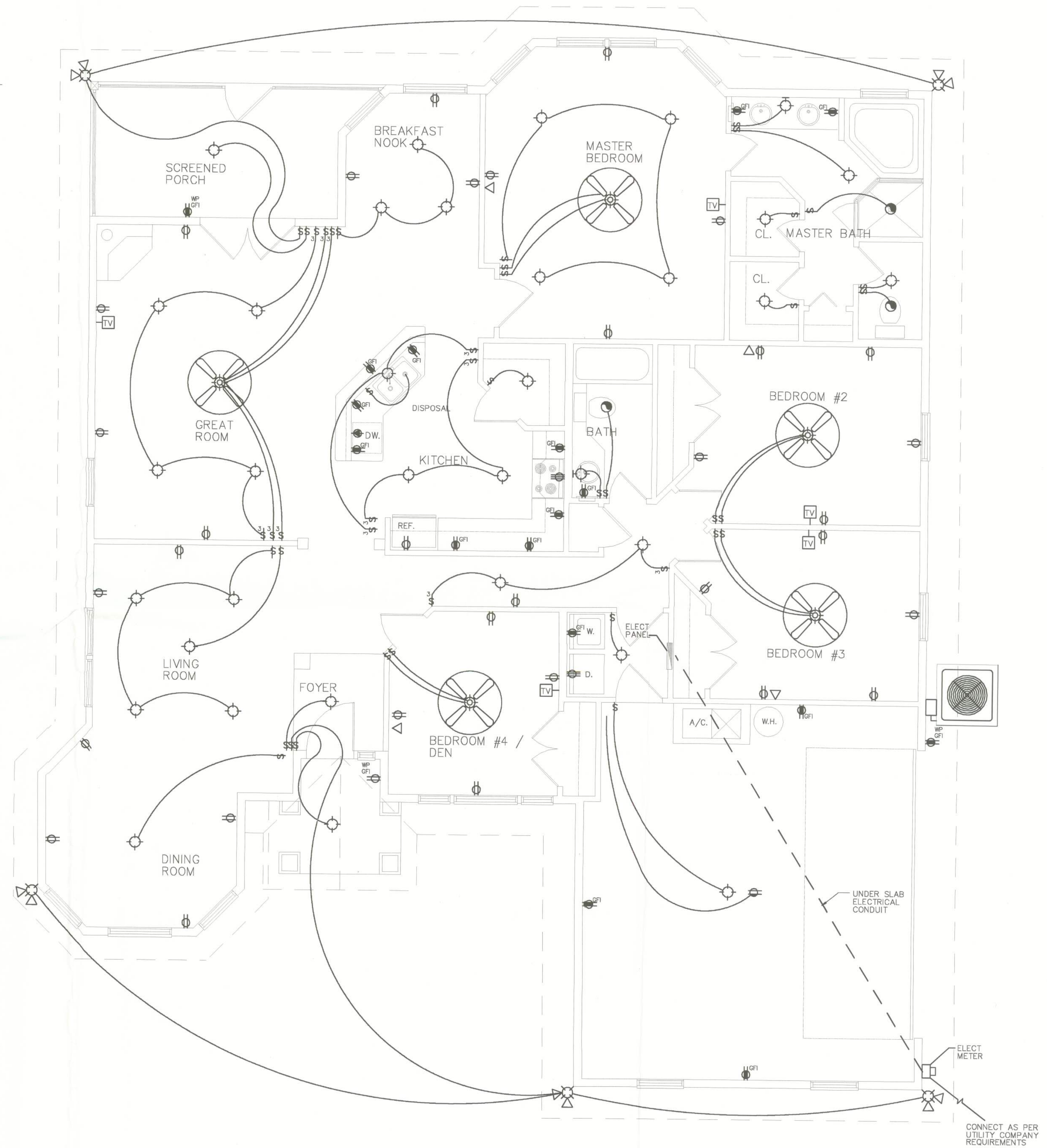
ELECTRICAL PLAN 1/4"=1'-0"
