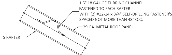
TYPICAL SIDE ELEVATION - EXTRA SIDE PANELS
