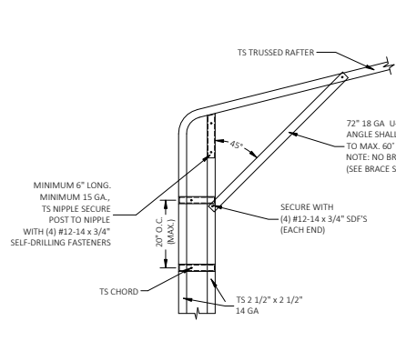
1B BOW EAVE RAFTER COLUMN CONNECTION DETAIL FOR HEIGHTS 16'-0" < TO ≤ 20'-0" SCALE: NTS
