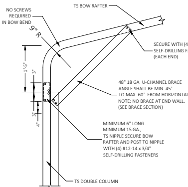
1A BOW EAVE RAFTER COLUMN CONNECTION DETAIL FOR HEIGHTS 14'-0" < TO ≤ 16'-0" SCALE: NTS
