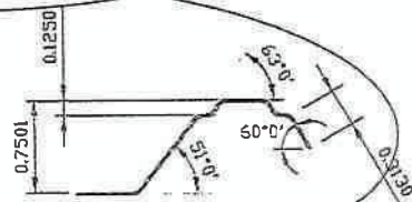
OVERLAP SIDE
