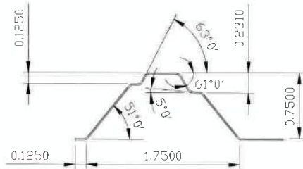
UNDERLAP SIDE
