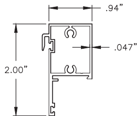
BOTTOM SASH TOP RAIL 6063-T5
