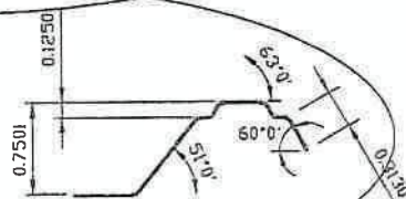
OVERLAP SIDE
