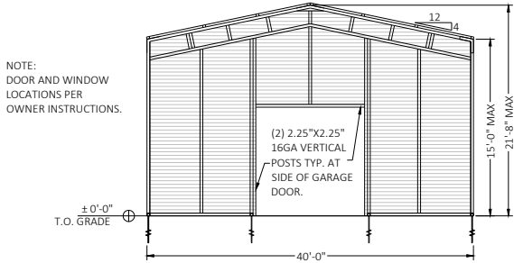
A-FRAME FRONT ELEVATION
