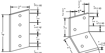
METAL CONNECTOR PLATE
