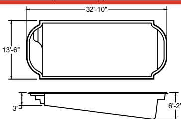
CLASSIC COVE - BHCC 11,300 Gal. Approx.
