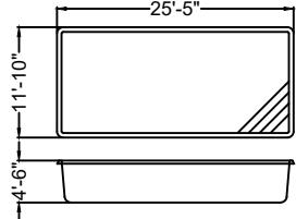
DELRAY - B 8,100 gal. approx.
