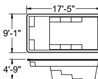
ENCHANTMENT 9.17 - NIV05 3,200 gal. approx.
