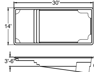
CORINTHIAN 14 - RT14 8,200 gal. approx.
