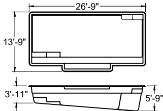
TUSCAN 14.27 - SYM08 7,900 gal. approx.
