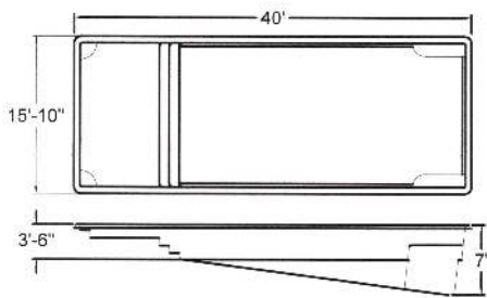
CORINTHIAN 16 - RT16 15,400 Gal. Approx.
