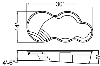
AXIOM 14/NEBULA - CRUL 8,000 gal. approx.
