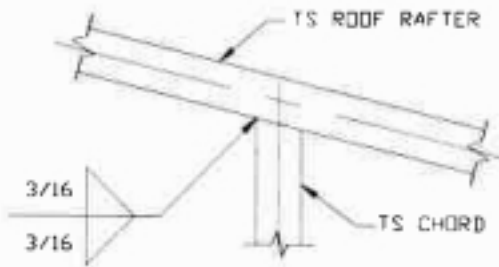
11 RAFTER TO CHORD CONNECTION DETAIL
