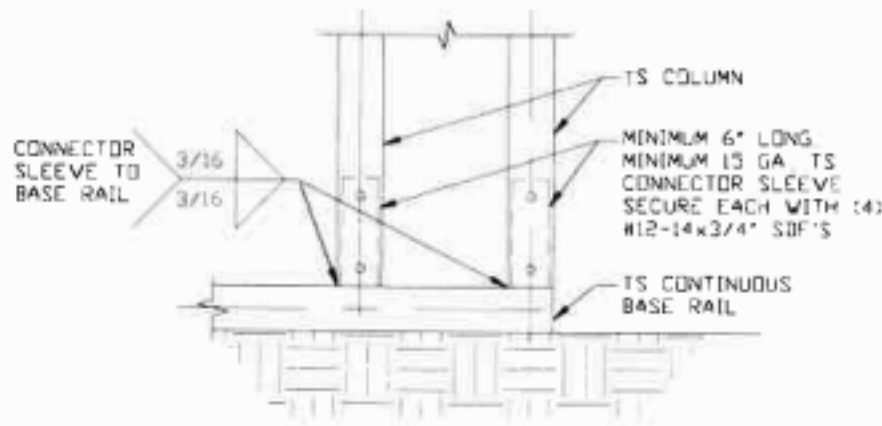
10 COLUMN/BASE RAIL CONNECTION DETAIL
