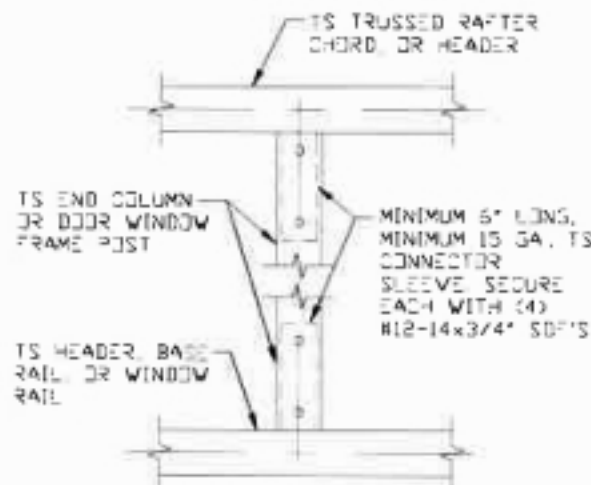
14 COLUMN TO HEADER, BASE RAIL CONNECTION DETAIL
