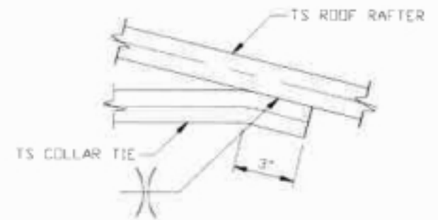
12 COLLAR TIE CONNECTION DETAIL
