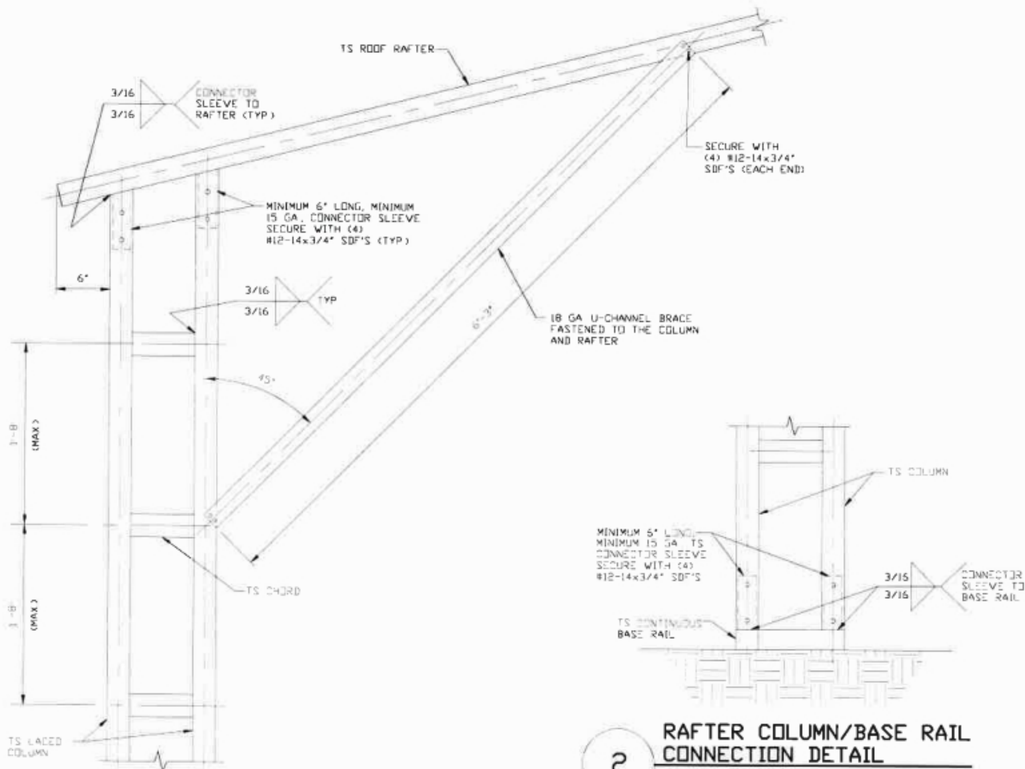
BOX EAVE RAFTER COLUMN CONNECTION DETAIL FOR HEIGHTS 16'-0" < TO ≤ 20'-0"
