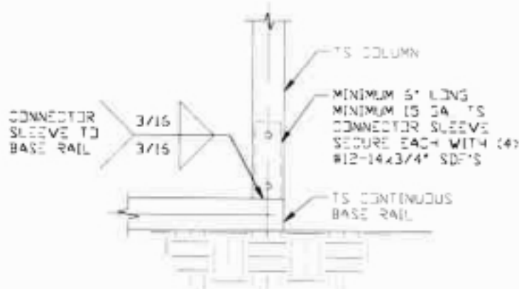
13 COLUMN/BASE RAIL CONNECTION DETAIL
