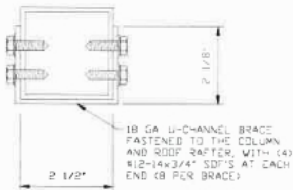
BRACE SECTION
