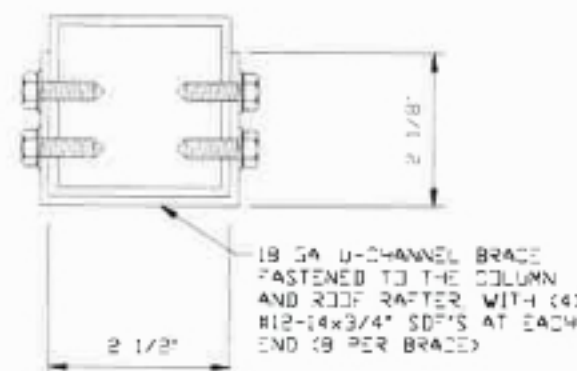
BRACE SECTION
