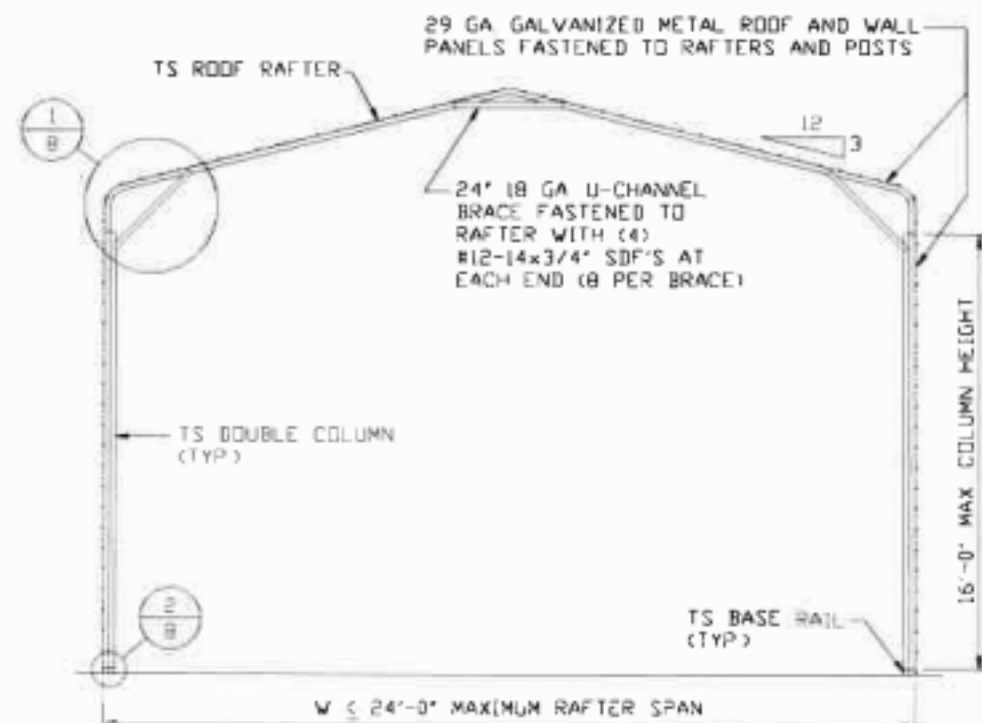
TYPICAL RAFTER/COLUMN END FRAME SECTION
