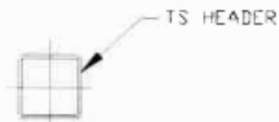
HEADER DETAIL FOR DOOR OPENINGS ≤ 12'-0'
