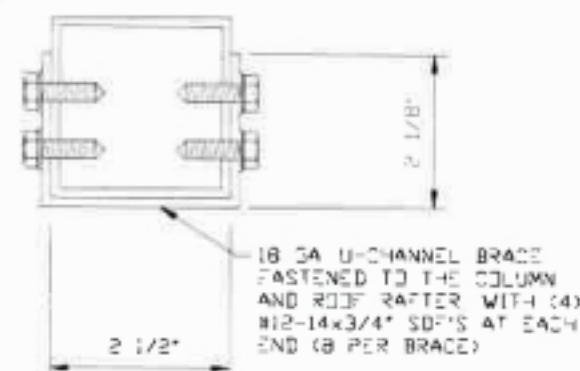
BRACE SECTION
