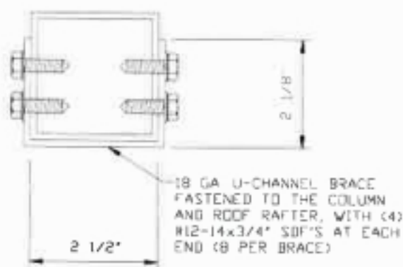
BRACE SECTION
