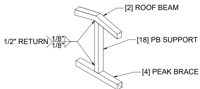
4. PB SUPPORT DETAIL
