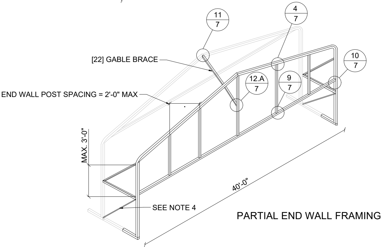
END WALL GABLES
