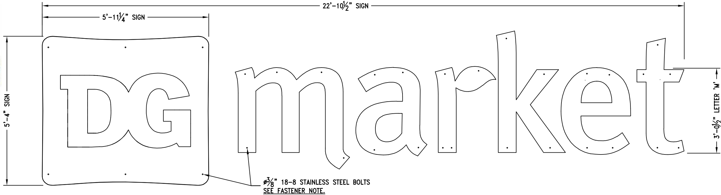
ELEVATION VIEW
