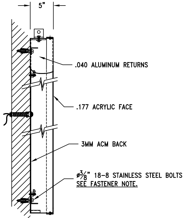
DETAIL VIEW-SIGN
