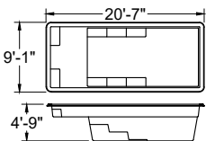
ENCHANTMENT 9.21 - NIV06 4,000 gal. approx.
