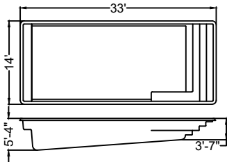
CLAREMONT - V 11,700 Gal. Approx.
