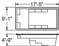
ENCHANTMENT 9.17 - NIV05 3,200 gal. approx.
