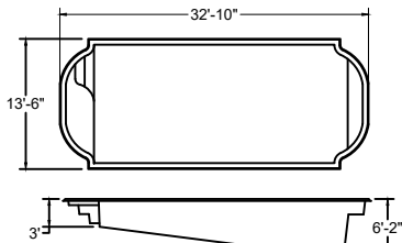
CLASSIC COVE - BHCC 11,300 Gal. Approx.
