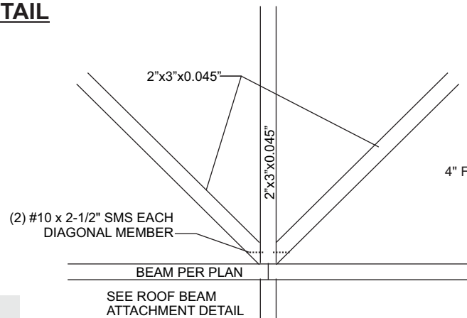
ROOF BEAM DIAGONAL ATTACHMENT
