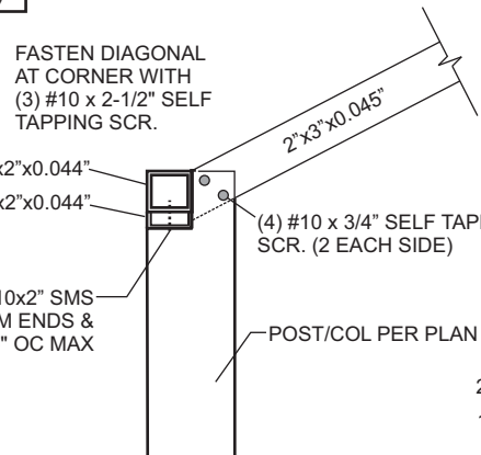
PURLIN TO POST (OPTION 1)
