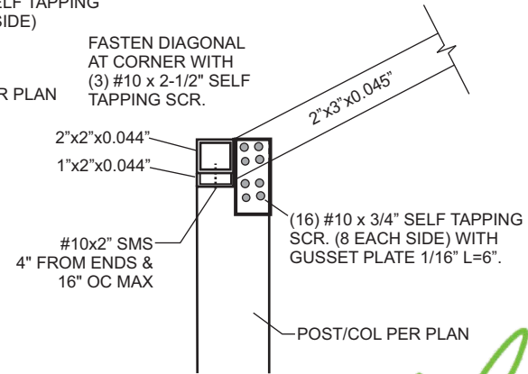
PURLIN TO POST (OPTION 2)
