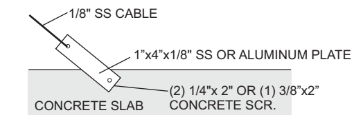
CABLE TO CONCRETE ANCHOR
