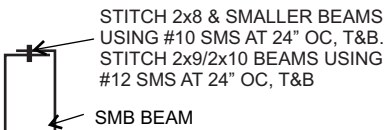
SMB DETAIL
