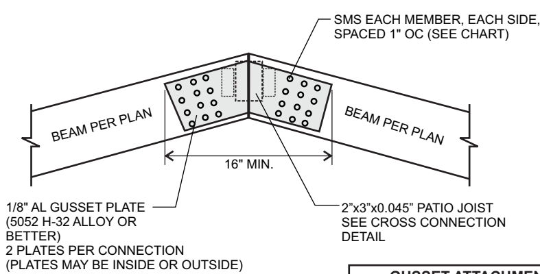
GUSSET DETAIL
