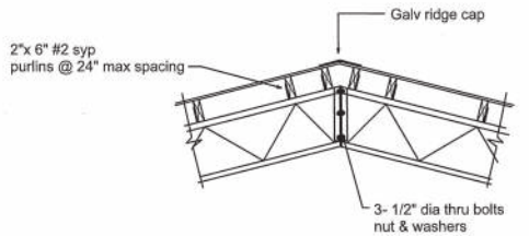
RIDGE CONNECTION DETAIL
