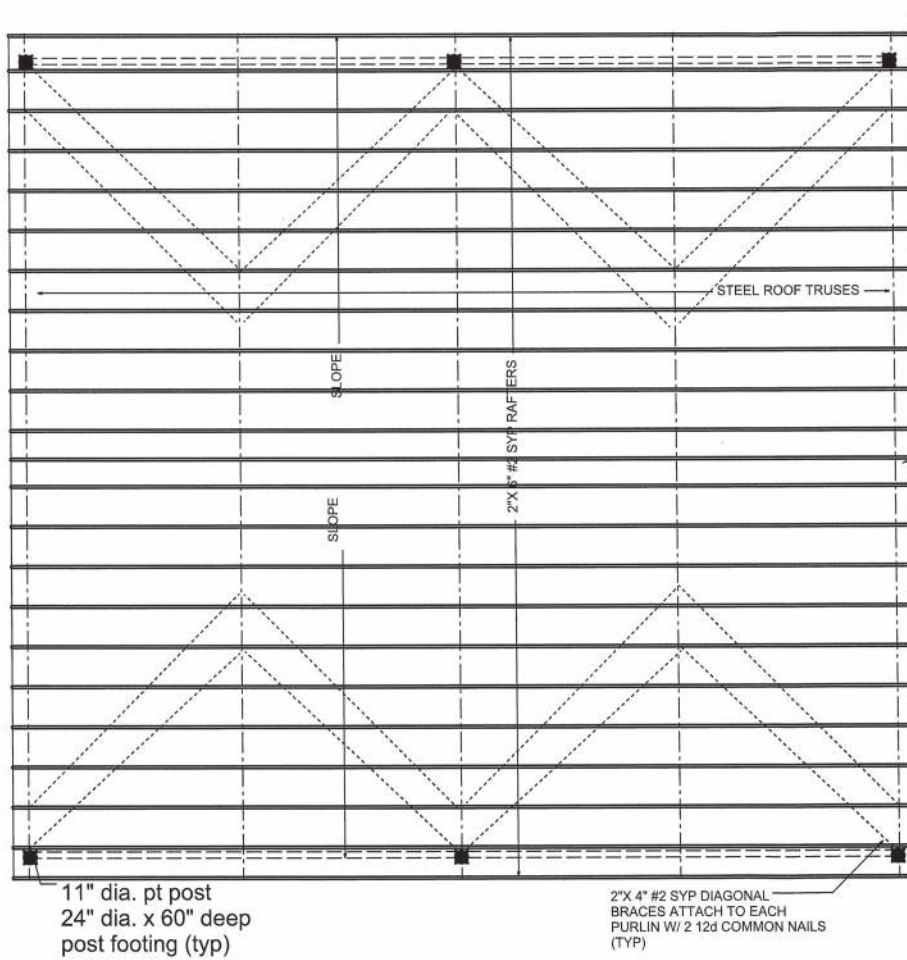
ROOF PLAN VIEW
