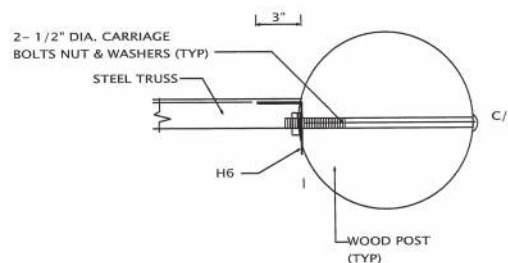
TRUSS TO POST DETAIL PLAN VIEW
