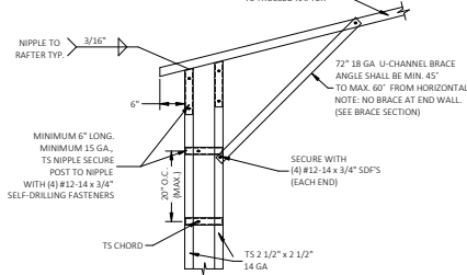
1B BOX EAVE RAFTER COLUMN CONNECTION DETAIL FOR HEIGHTS 16'-0" < TO ≤ 20'-0" SCALE: NTS
