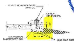
CONCRETE SLAB CONNECTION
