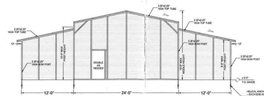
"A" FRAME 24 FT BARN REAR ELEVATION
