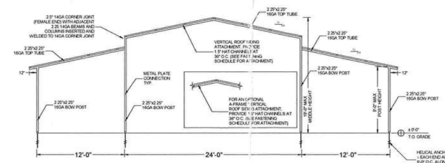
"A" FRAME 24 FT BOW SECTION BARN
