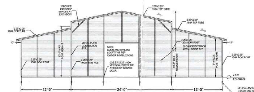
"A" FRAME 24 FT BARN FRONT ELEVATION
