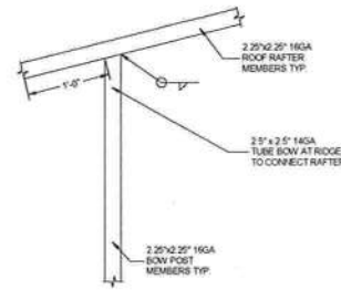
TEE SPLICE CONNECTION
