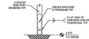
BOW/BASE RAIL SPLICE CONNECTION
