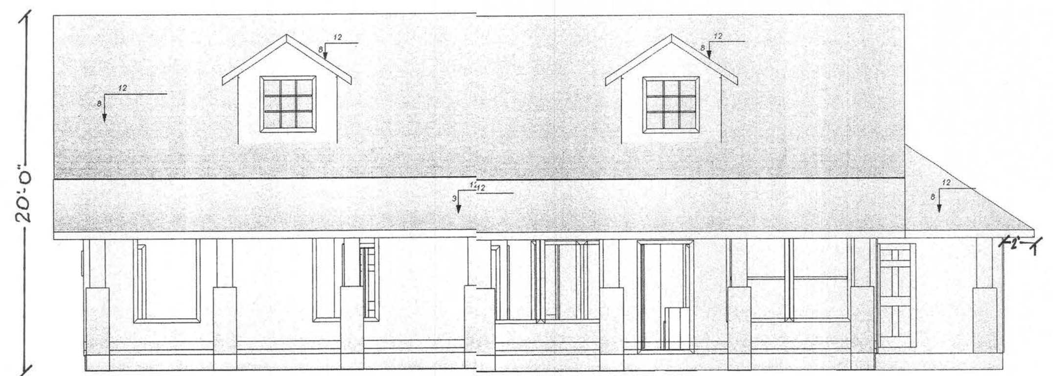
FRONT ELEVATION
