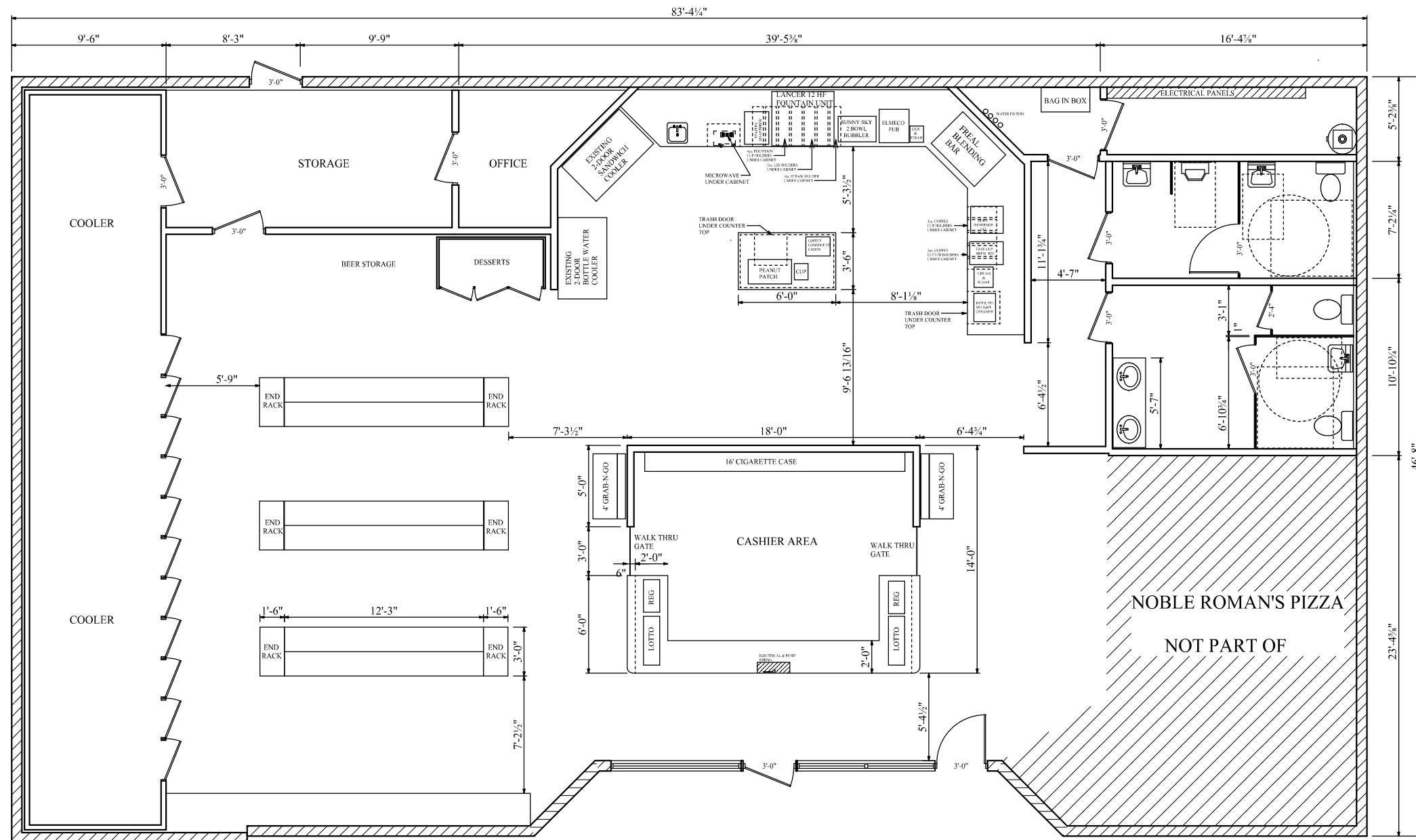
INLAND STORE #341 PROPOSED FLOOR LAYOUT 08-25-22 SCALE: 1/8" = 1'-0"
