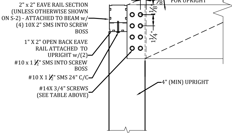
D S-3 UPRIGHT TO BEAM CONNECTION - ALL WIND ZONES SCALE: NTS
