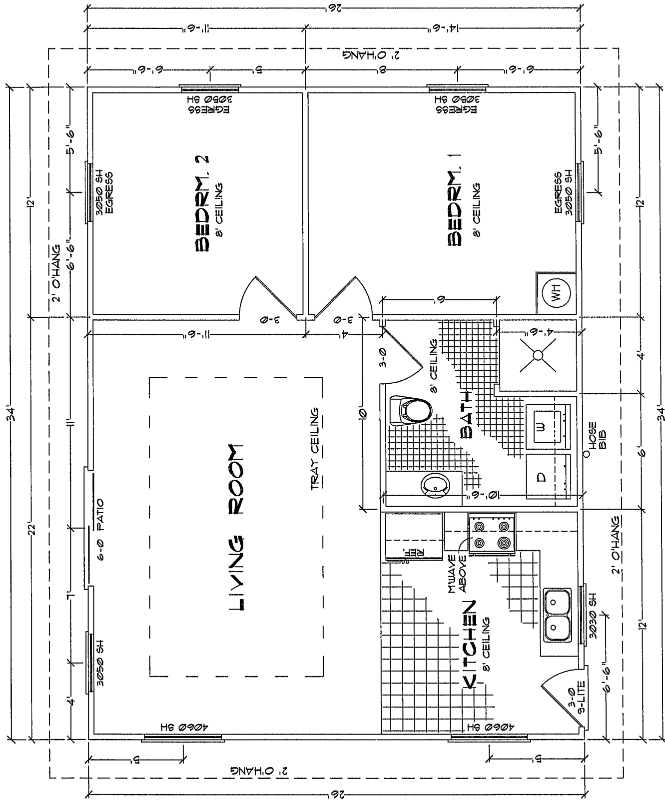
FLOOR PLAN 884 SQ FT
