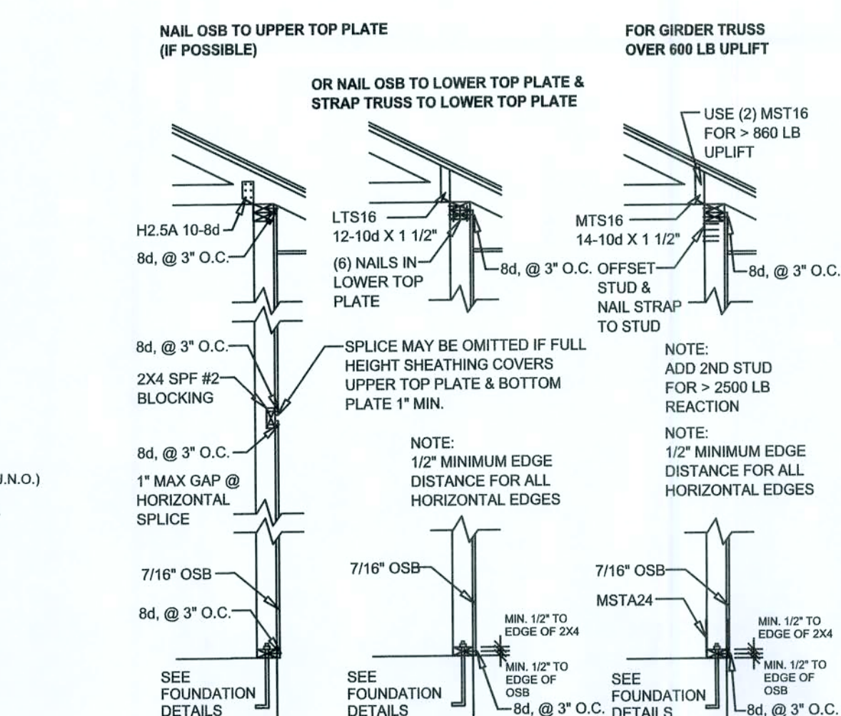
W61 - SHEATHING NAILING FOR TRUSS UPLIFT SCALE: 1/2" = 1'-0"
