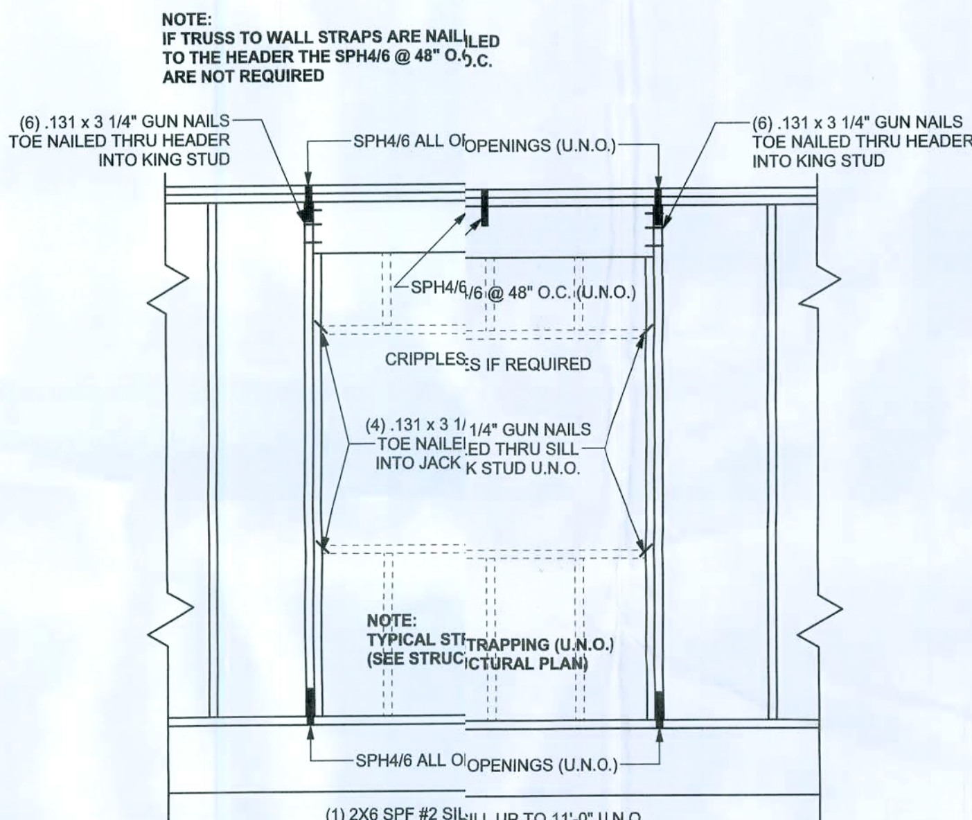
TYPICAL HEADER STRAPPING DETAIL 4'-0" OR LESS SCALE: 1/2" = 1'-0"
