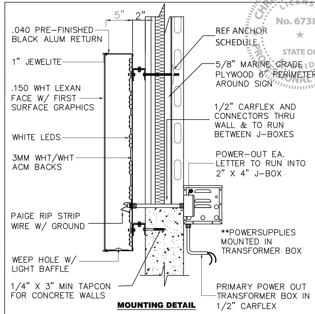
MOUNTING DETAIL
