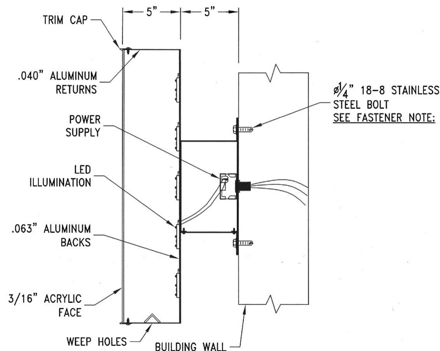
CHANNEL LOGO / LETTER DETAIL VIEW
