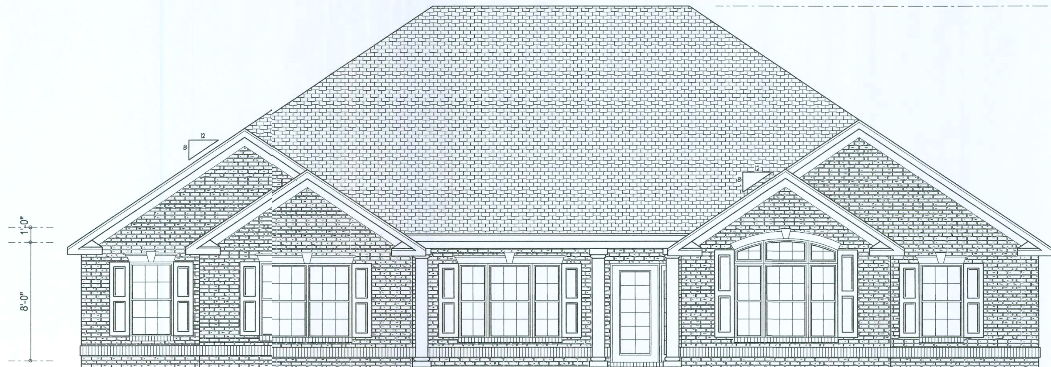
FRONT ELEVATION
