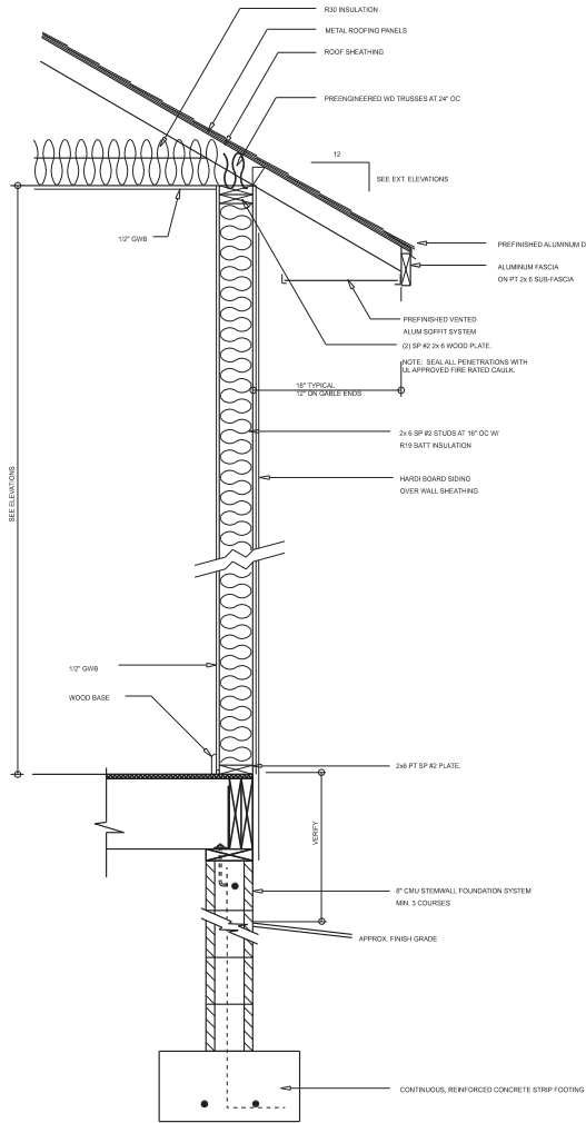
TYPICAL WALL SECTION SCALE: NOT TO SCALE
