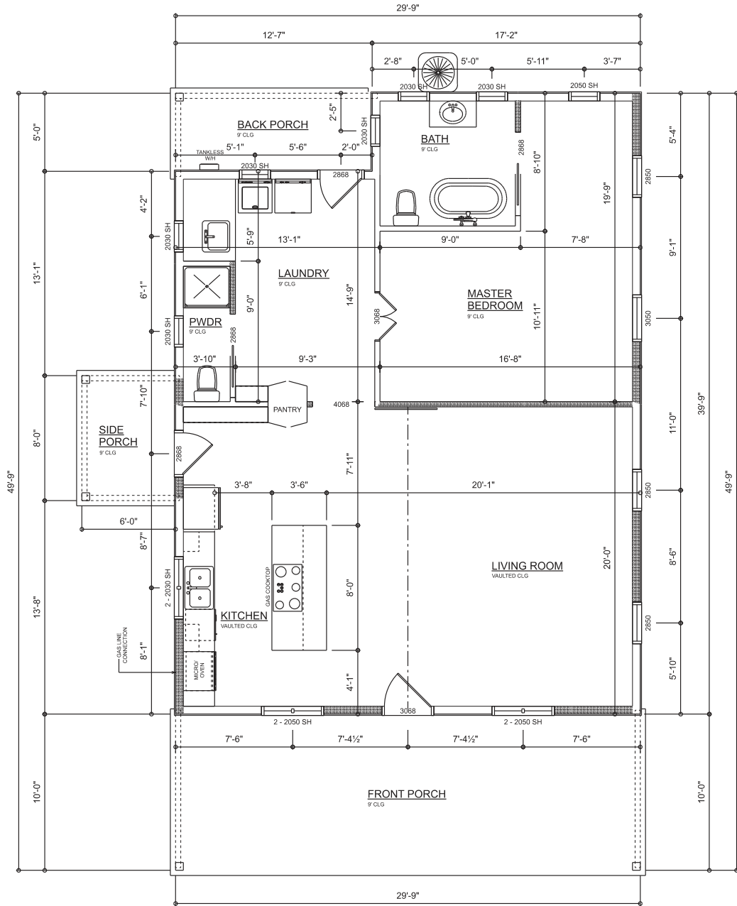
DIMENSIONED FLOOR PLAN SCALE: 1/4\"/>
