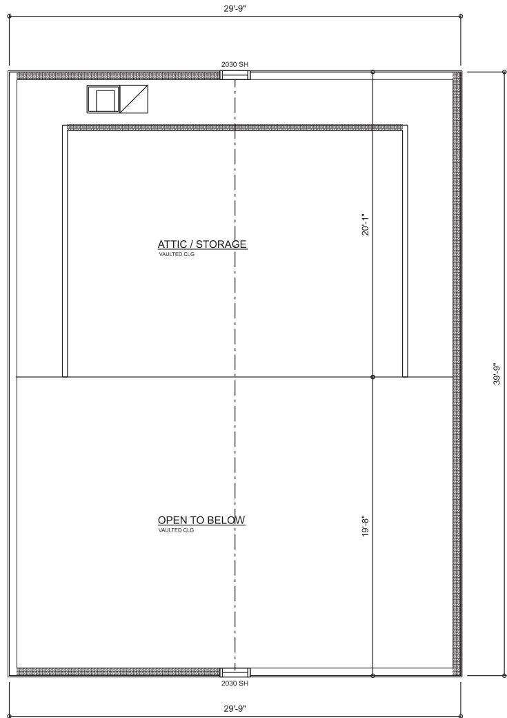
LOFT PLAN SCALE: 1/4\"/>
