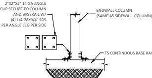
2C ENDWALL COLUMN/BASE RAIL CONNECTION DETAIL SCALE: NTS
