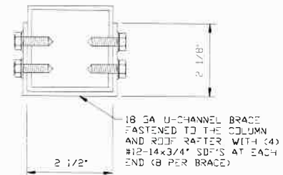
BRACE SECTION
