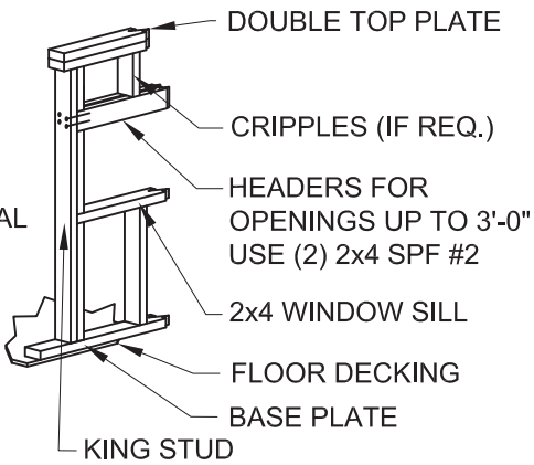
2A WINDOW HEADER DETAIL FOR SIDE WALLS
