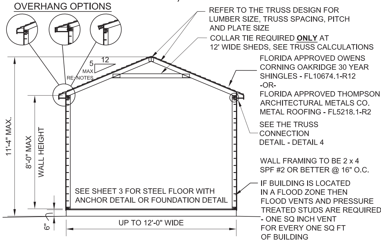
1 BUILDING SECTION
