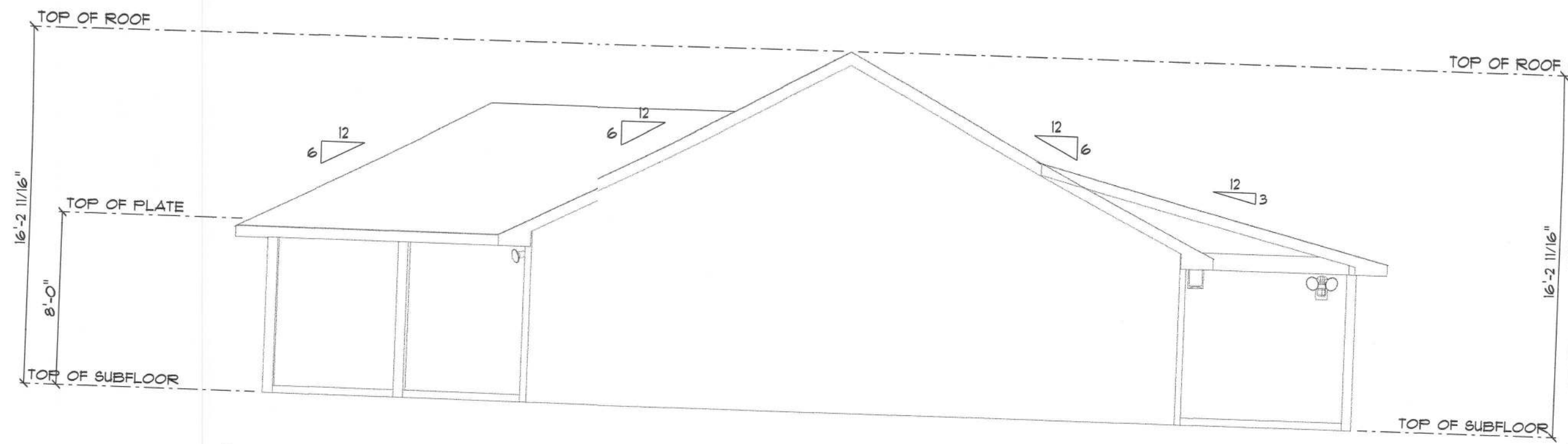
Left Elevation
