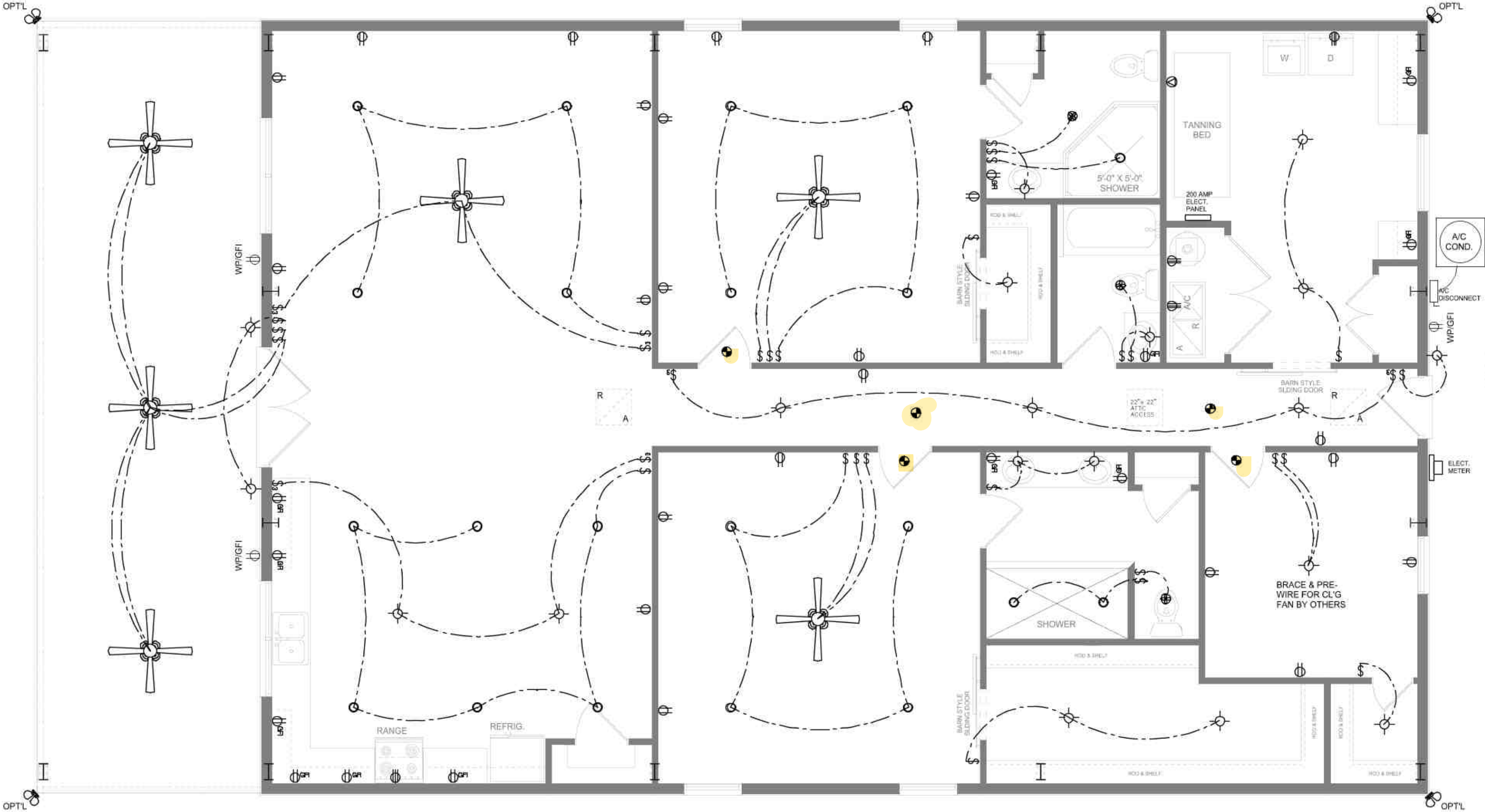
ELECTRICAL PLAN SCALE: 1/4\"/>
