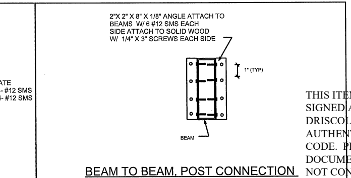
BEAM TO BEAM, POST CONNECTION
