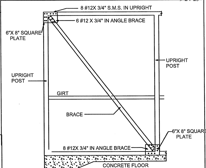
K- BRACING CONNECTION DETAIL N.T.S.
