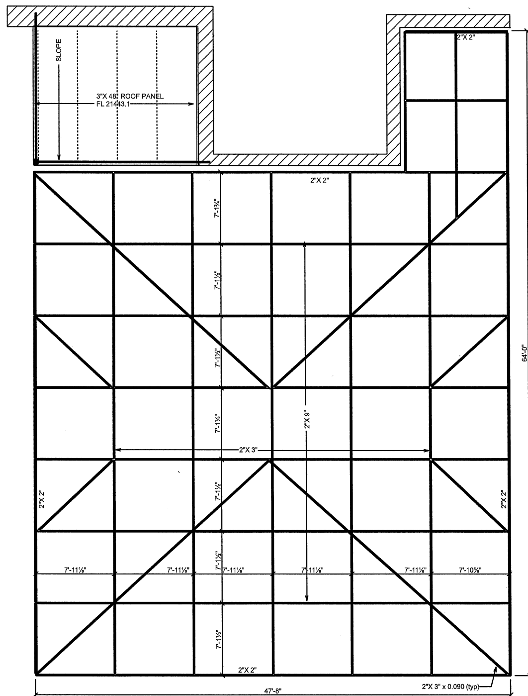
PLAN VIEW
