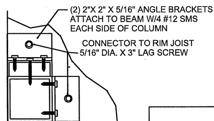
CORNER POST DETAIL PLAN VIEW
