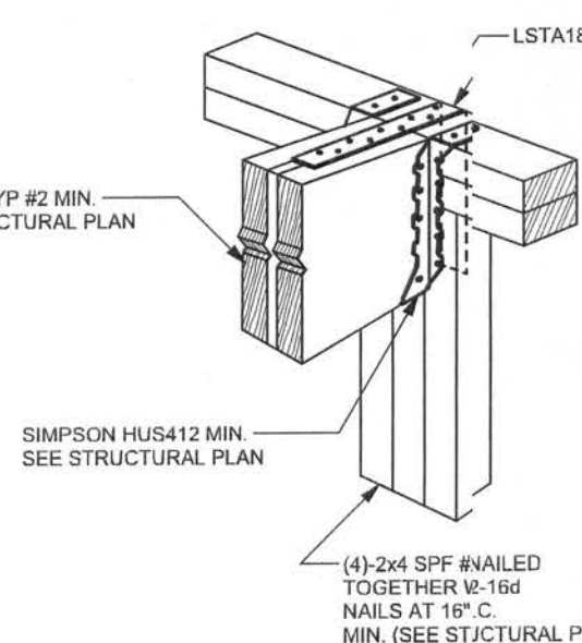
BEAM MID-WALL CONNECTION DETAIL SCALE: N.T.S.
