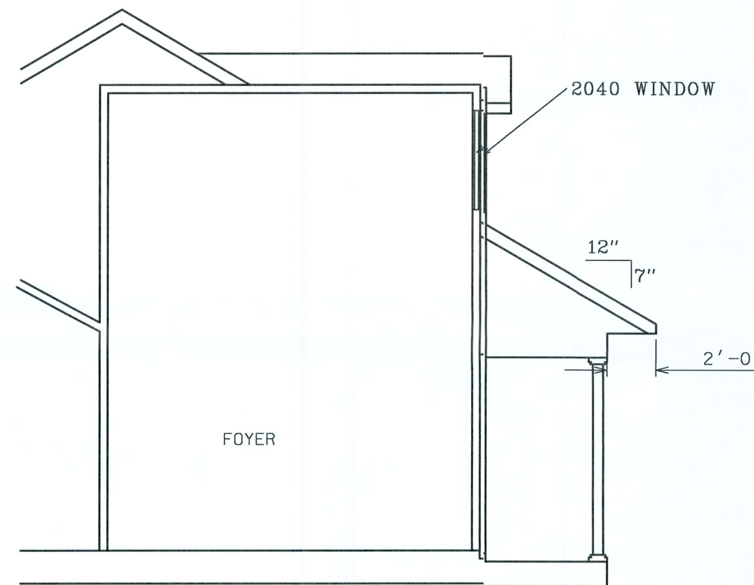
FOYER DETAIL (4/7)
