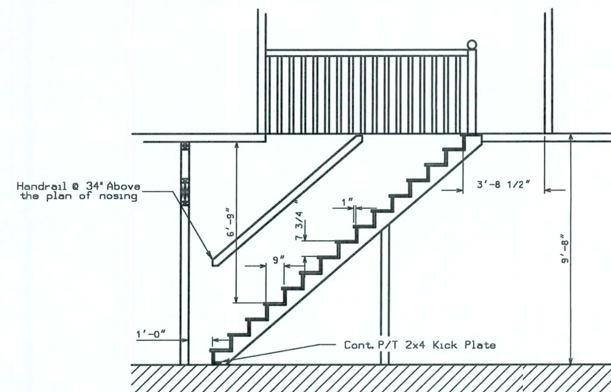
STAIR DETAIL (6/7)
