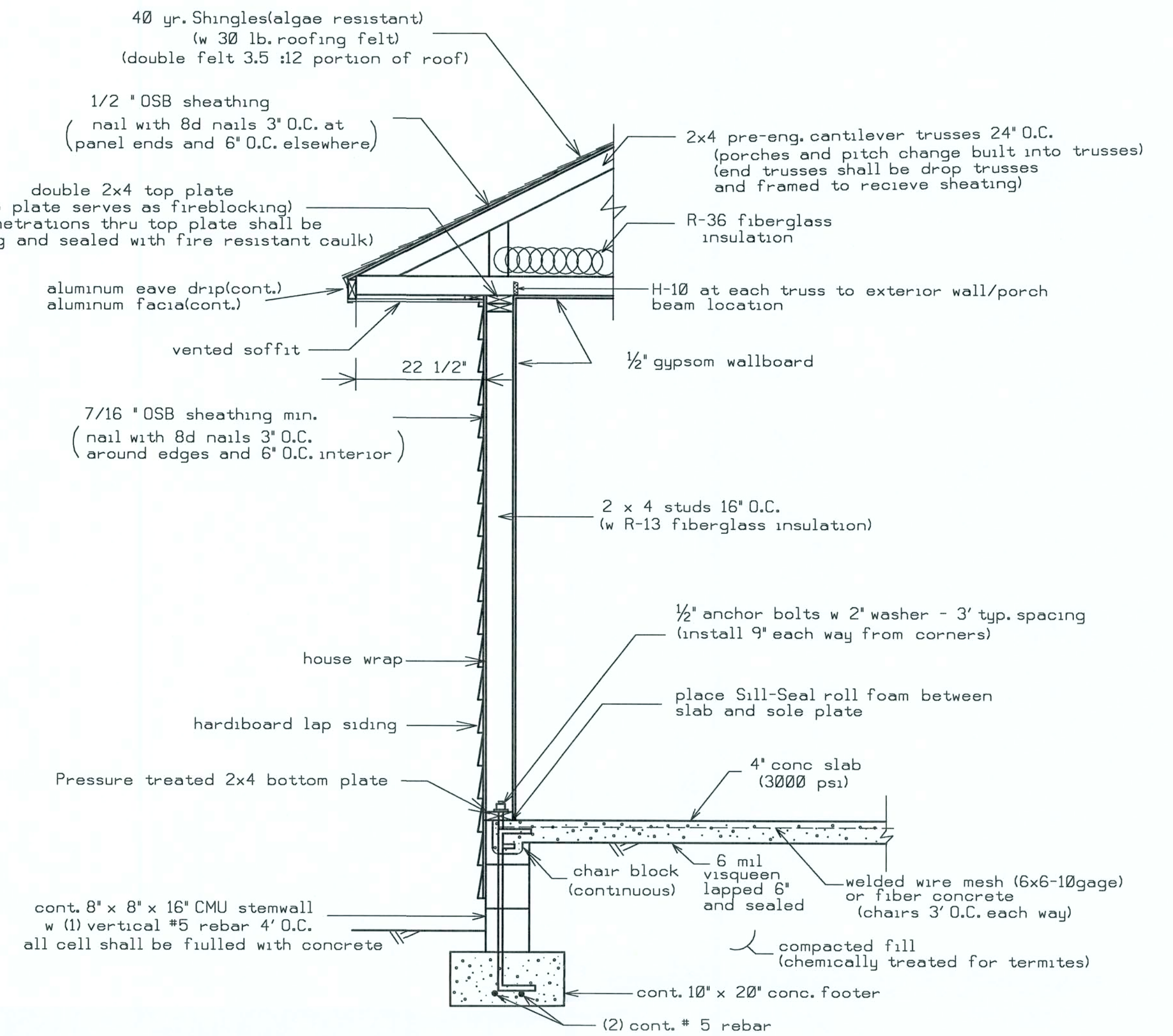
FOOTER DESIGN 1000 PSF
