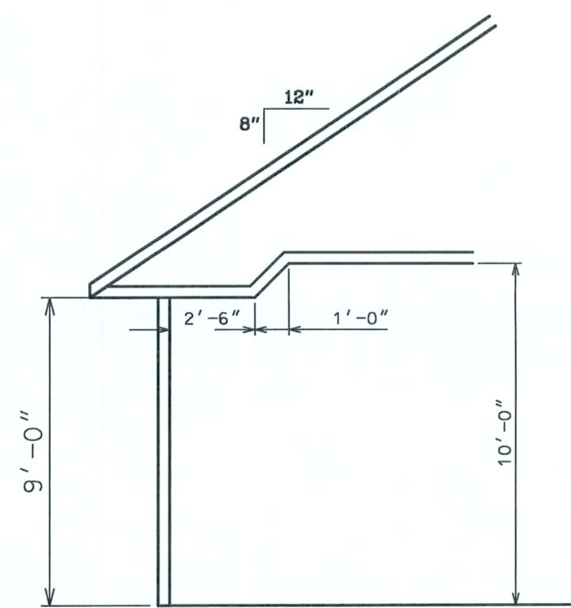
FAMILY ROOM (3/7)
