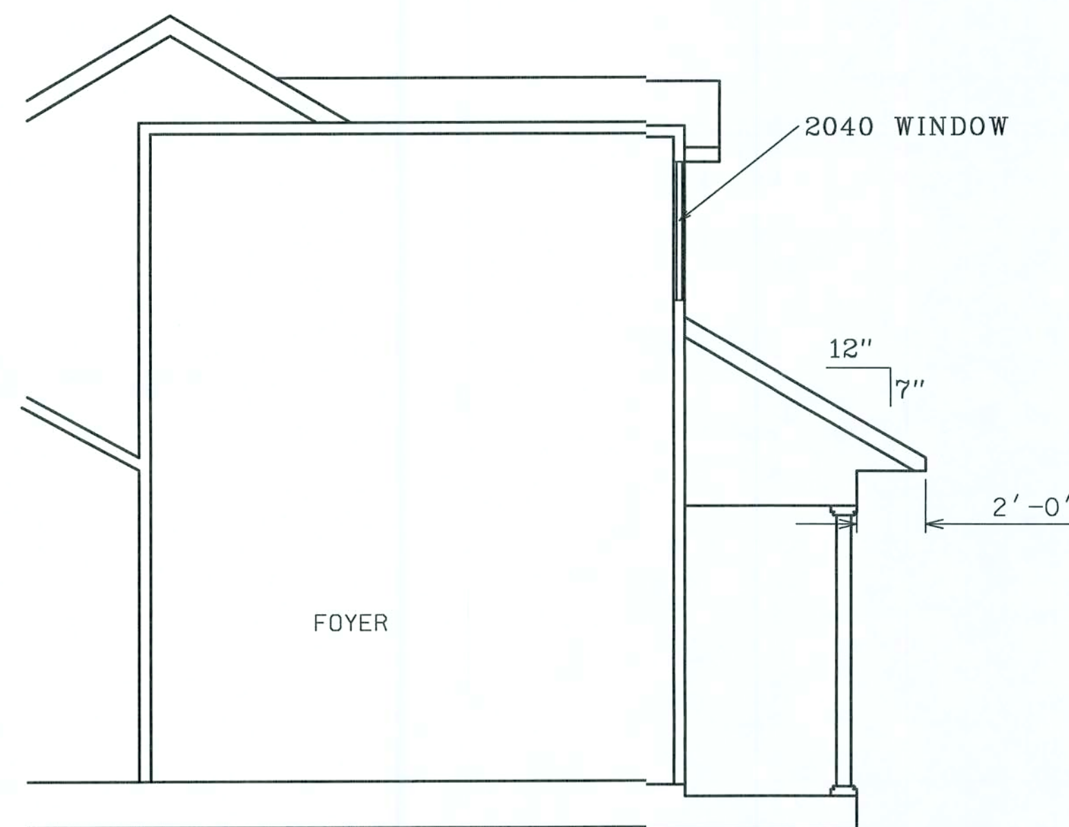
FOYER DETAIL (4/7)
