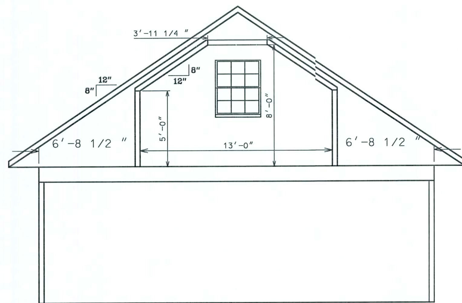
BONUS ROOM (1/7)
