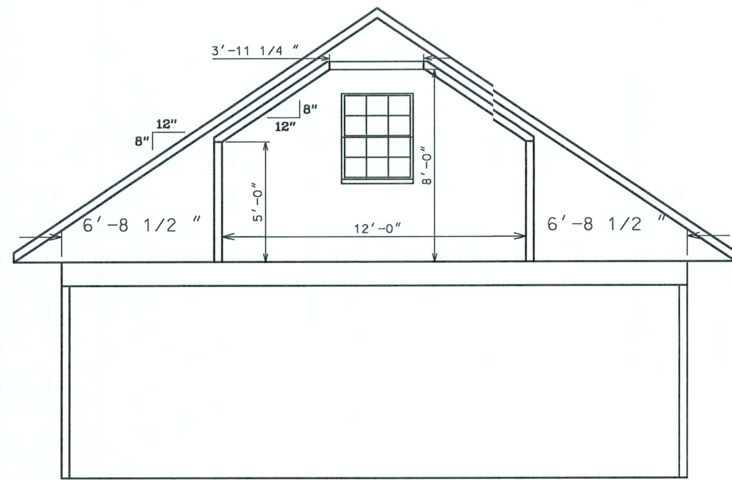
BONUS ROOM (1/7)
