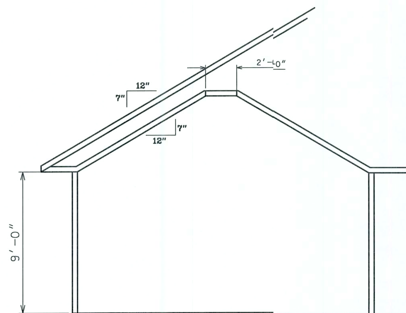
FAMILY ROOM (2/7)
