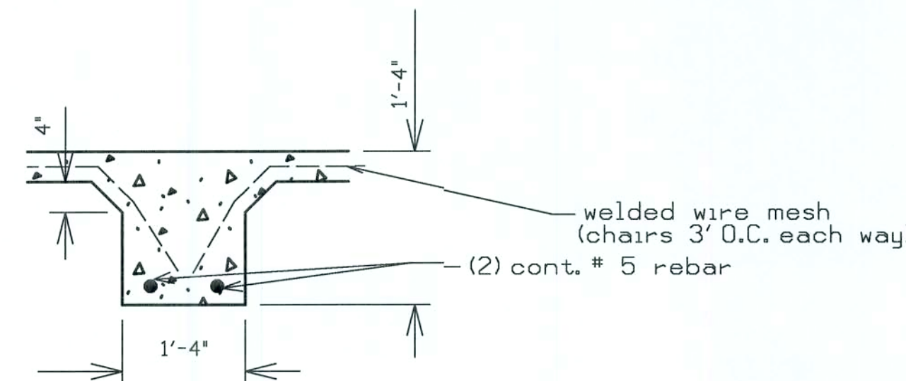
MONOLITHIC FOUNDATION (5/7)
