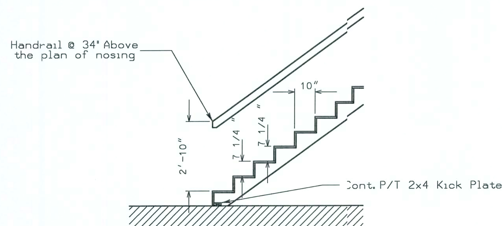
STAIR DETAIL (NTS)
