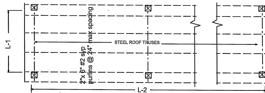
PLAN VIEW POST SPACING
