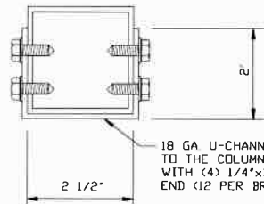
BRACE SECTION
