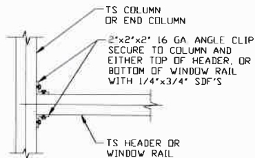
COLUMN OR WINDOW RAIL/ WALL GIRT TO POST CONNECTION DETAIL
