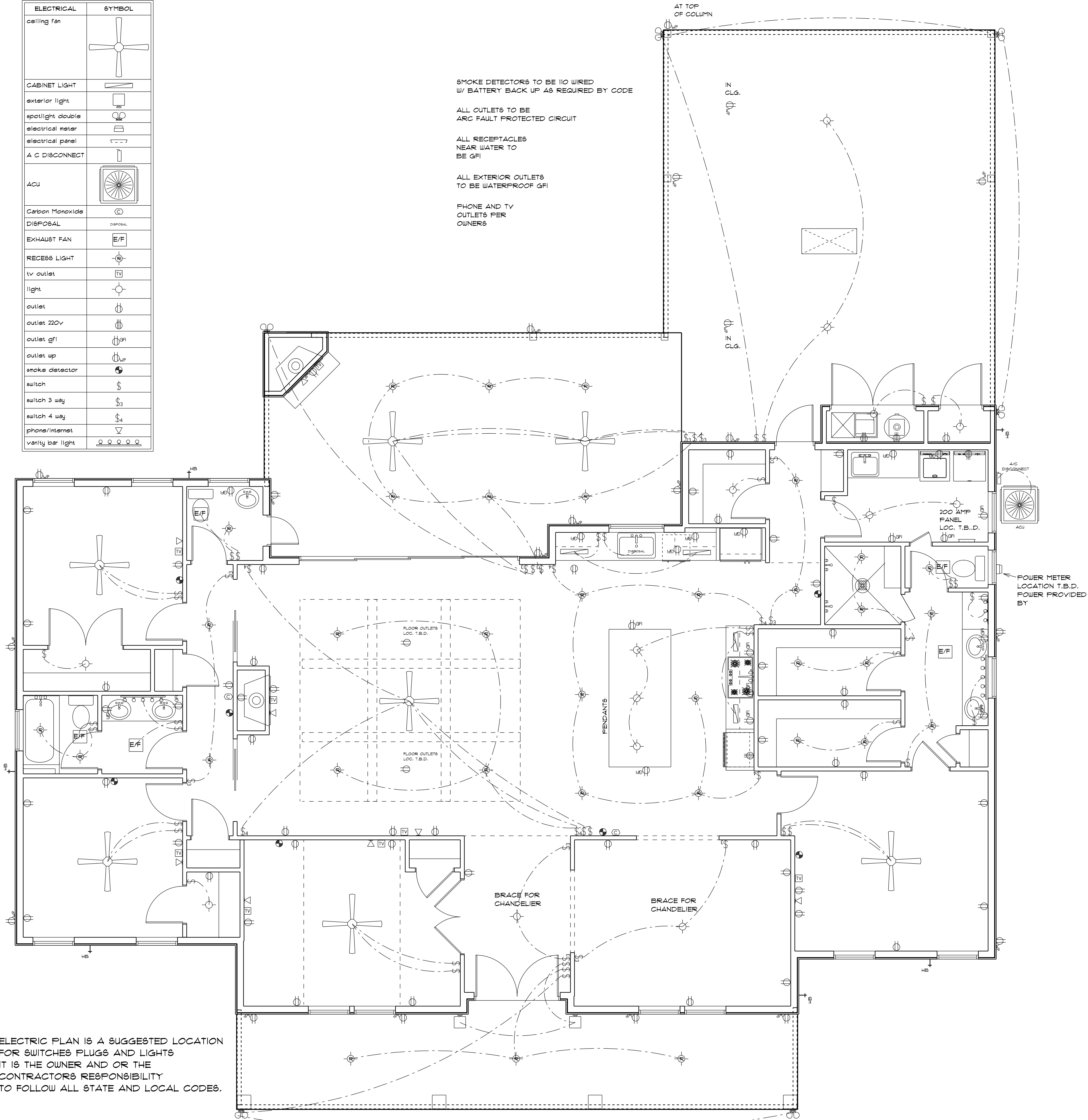
ELECTRICAL PLAN
