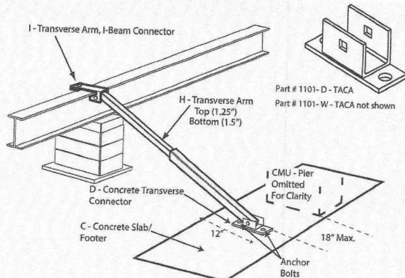
Model # 1101 TC "V"
