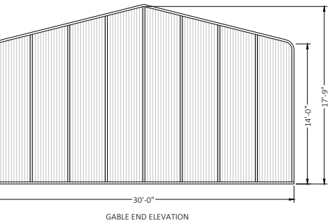
REGULAR STYLE BUILDING
