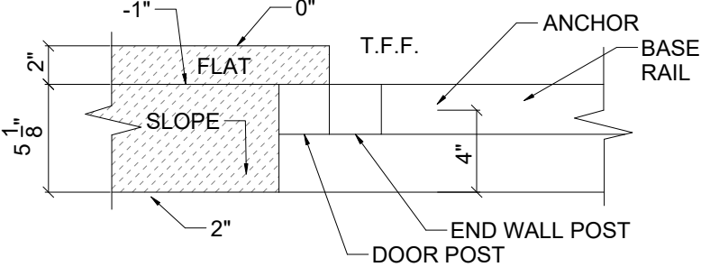
12GA SECTION A-A
