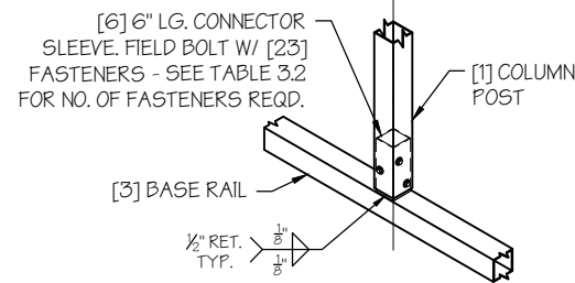
BASE DETAIL SCALE: NTS
