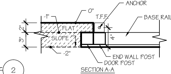
OVERHEAD DOOR NOTCH DETAIL
