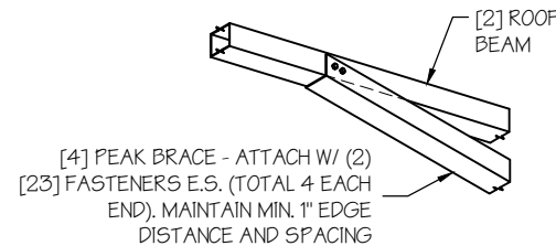
PEAK BRACE CONNECTION DETAILS SCALE: NTS
