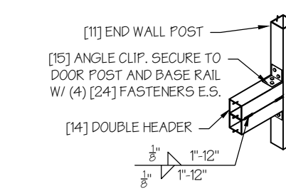
DOUBLE HEADER - END WALL POST CONN. DETAIL
