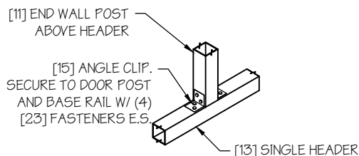
END WALL POST ABOVE HEADER CONN. DETAIL
