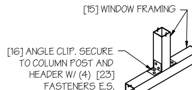
TYP. WINDOW FRAMING CONN. DETAIL
