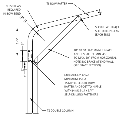
1A BOW EAVE RAFTER COLUMN CONNECTION DETAIL FOR HEIGHTS 14'-0" < TO ≤ 16'-0" SCALE: NTS
