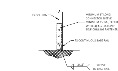
2 RAFTER POST/BASE RAIL CONNECTION DETAIL SCALE: NTS
