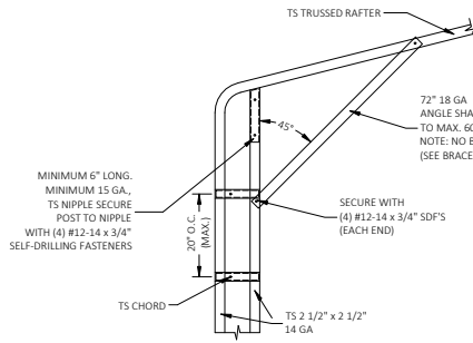
1B BOW EAVE RAFTER COLUMN CONNECTION DETAIL FOR HEIGHTS 16'-0" < TO ≤ 20'-0" SCALE: NTS
