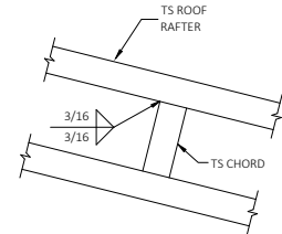
3 RAFTER TO CHORD CONNECTION SCALE: NTS
