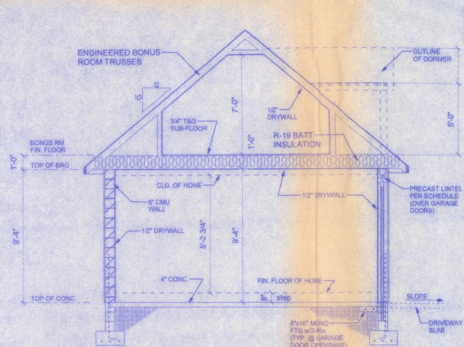
B SECTION THROUGH (GARAGE) SCALE: 1/4" = 1'-0"
