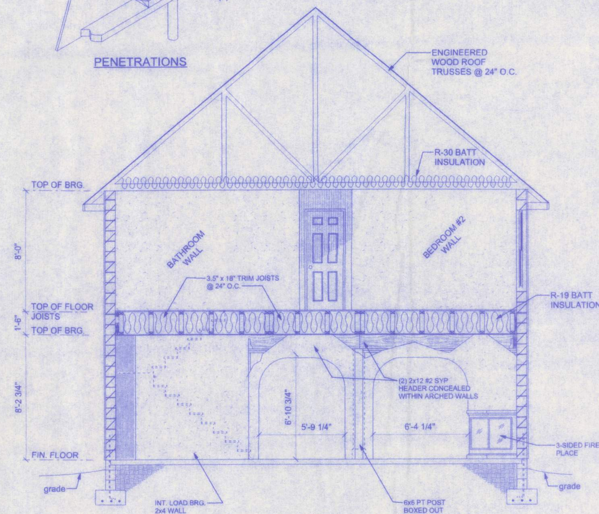
C SECTION THROUGH (RIGHT VIEW) SCALE: 1/4" = 1'-0"
