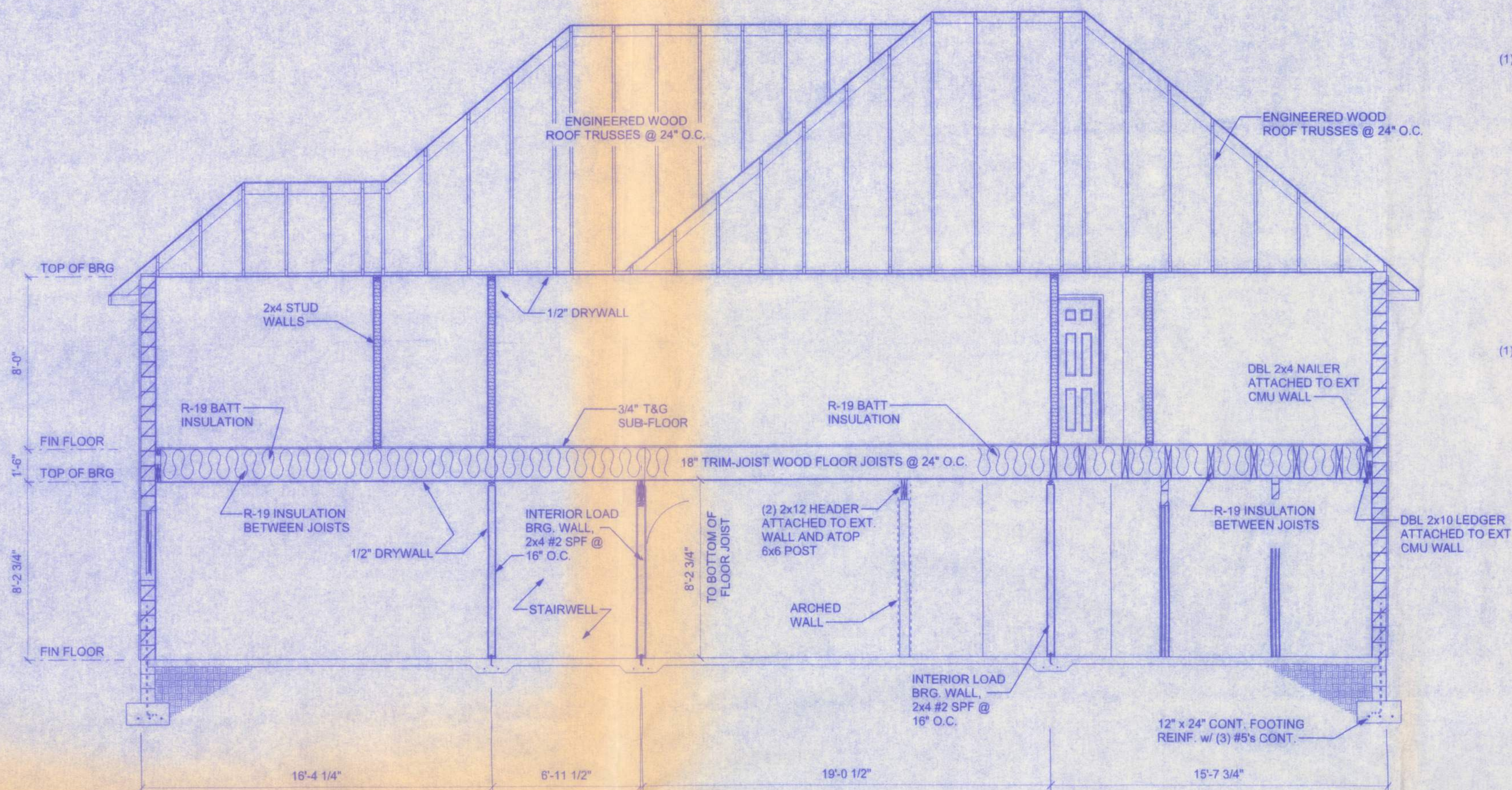
A SECTION THROUGH (FRONT VIEW) SCALE: 1/4" = 1'-0"
