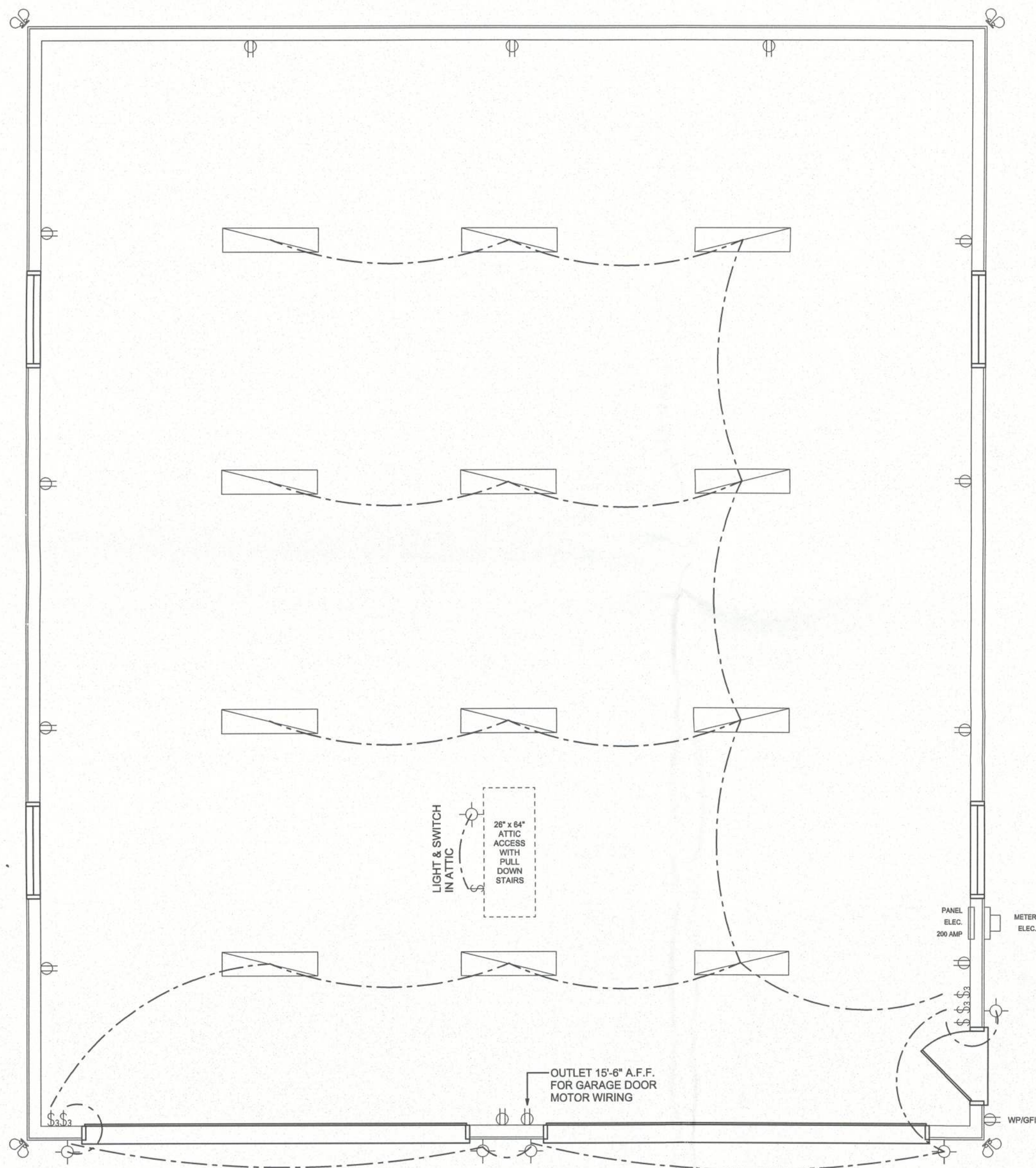
ELECTRICAL PLAN SCALE: 1/4" = 1'-0"
