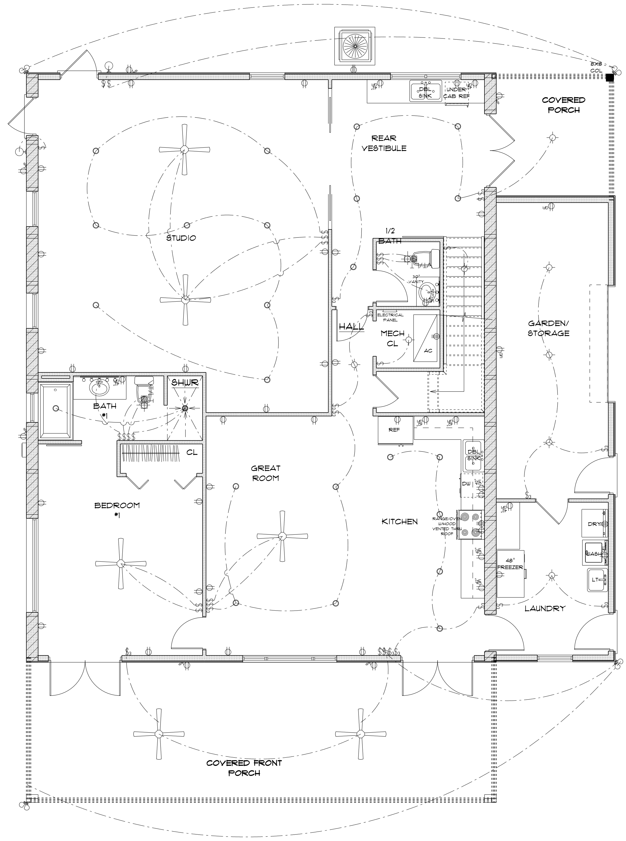
* ELECTRIC PLAN * SCALE : 1/4" = 1'-0"
