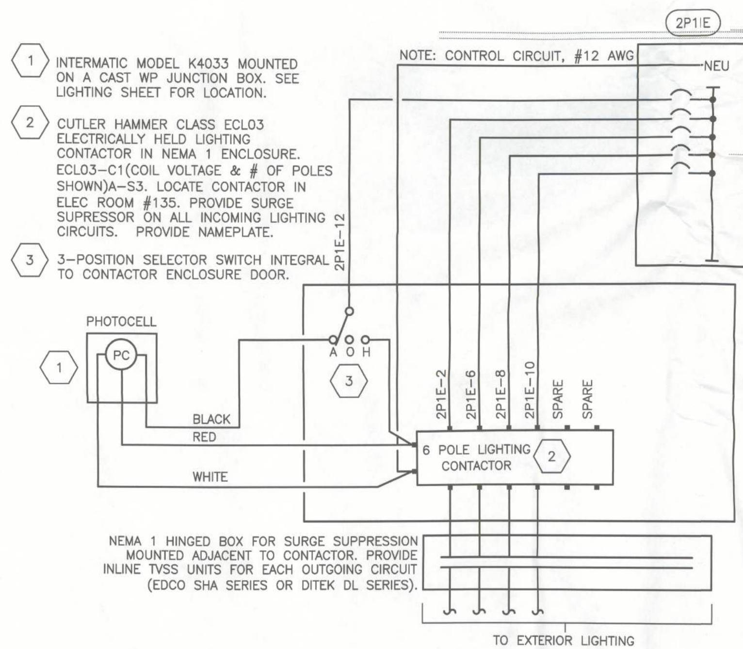
EXTERIOR LIGHTING CONTROL DIAGRAM NOT TO SCALE
