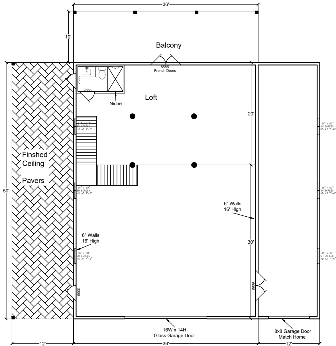
Floor Plan
